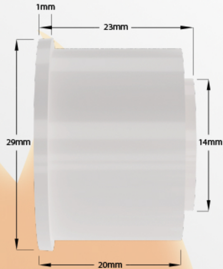
Capillary Adaptor
