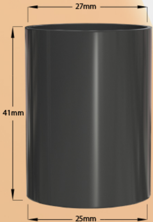
Side Elevation
